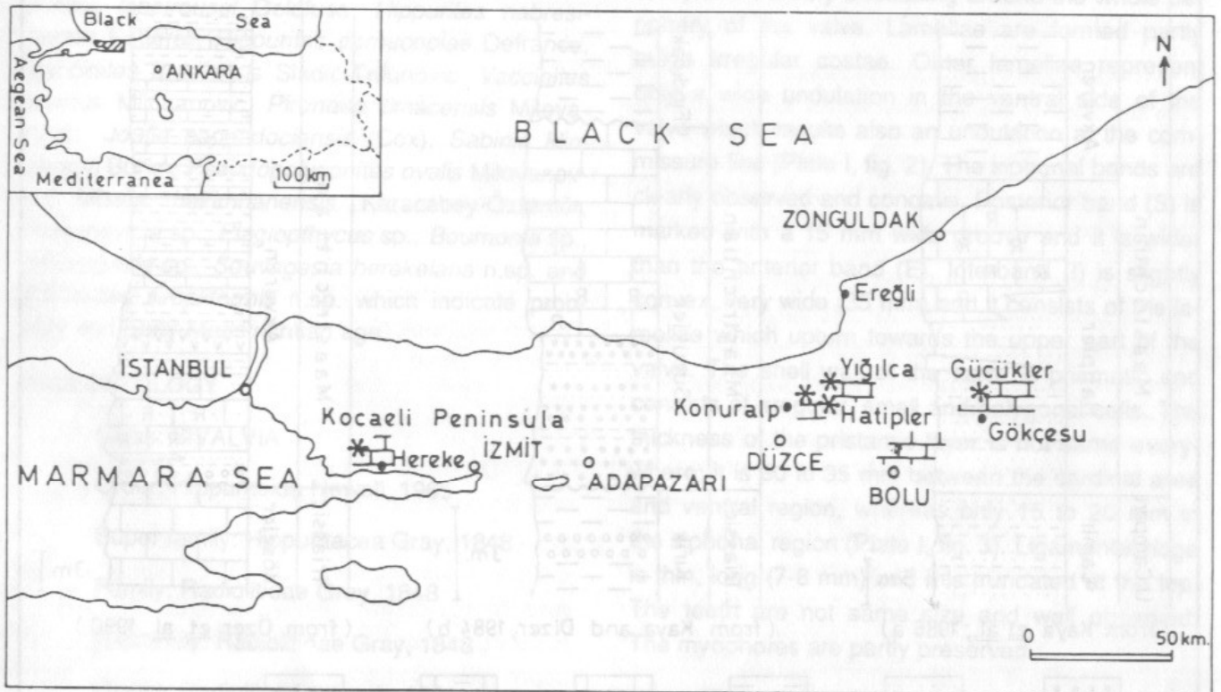
Fig. 1- Map showing the distribution of the late Senonian rudistid formations (hachured) and the localities of the new species in western Pontides and Kocaeli Peninsula.
