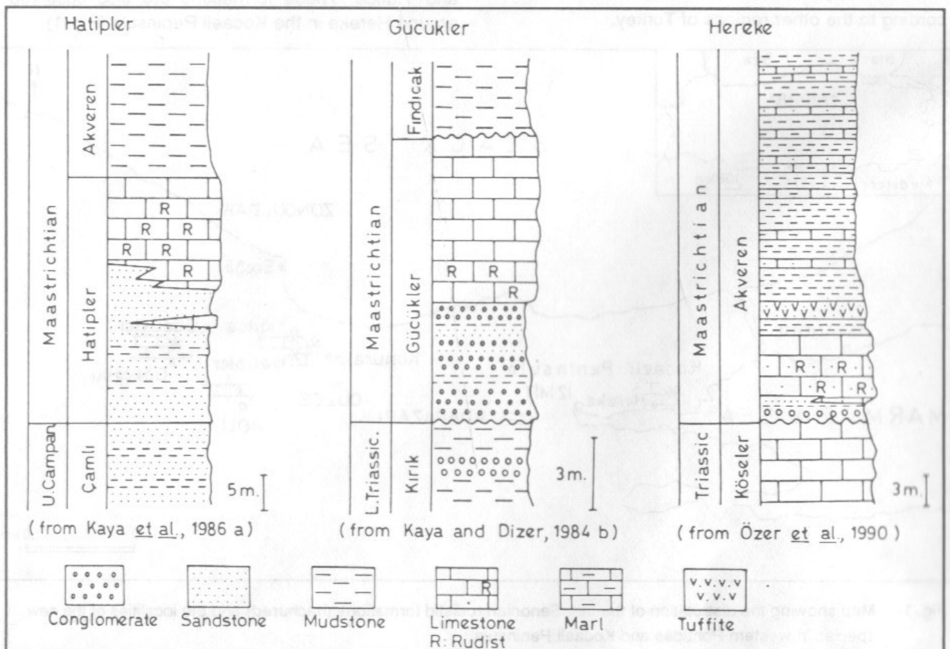
Fig. 2- Columnar sections of the rudistid localities.
